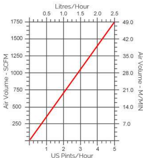
Rockdrill Oil Consumption
